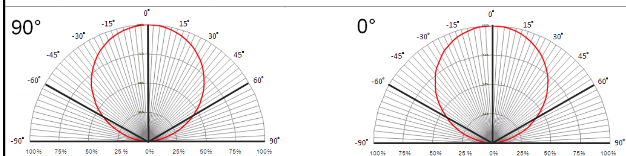
Directive Characteristics
