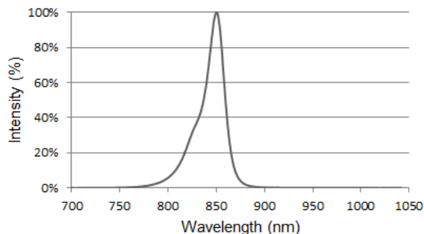
Relative Spectral Emission
