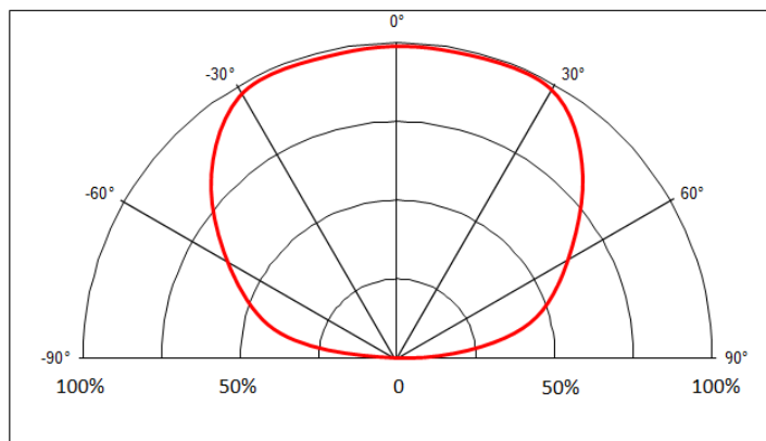
Relative Sensitivity VS. Angular Displacement
